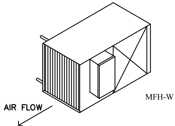
HOT WATER COIL LEFT HAND CONNECTION.
